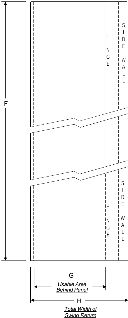
Front View of Swing Return
