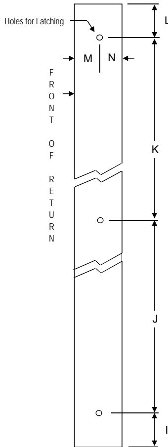
Side View of Swing Return
